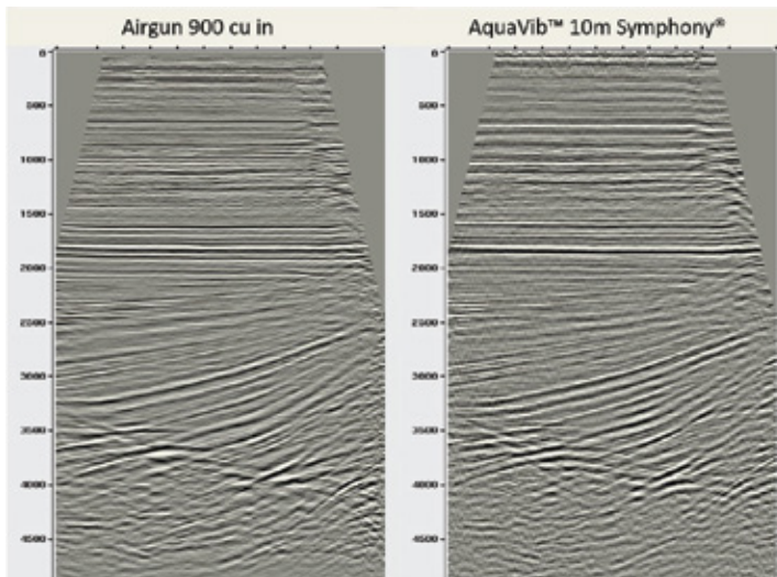
900 ci Airgun results; AquaVib™ 10m Symphony results
